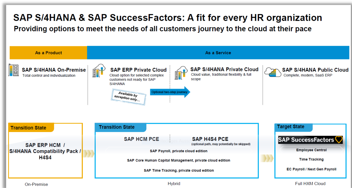
Abbildung 1: Deployment-Modelle (SAP)
